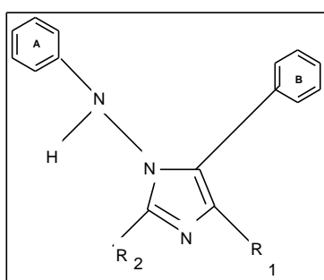
Figure 1. Parent skeleton of Anti-HIV 5-phenyl-1-H-imidazole
