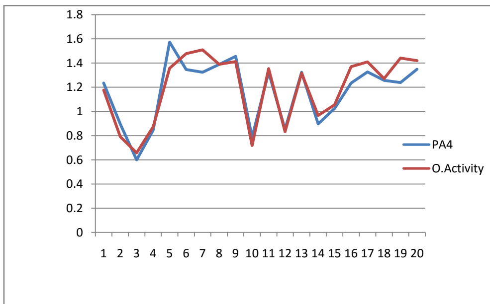
Fig 2. Graphical presentation of Best Model (PA4) of set A
