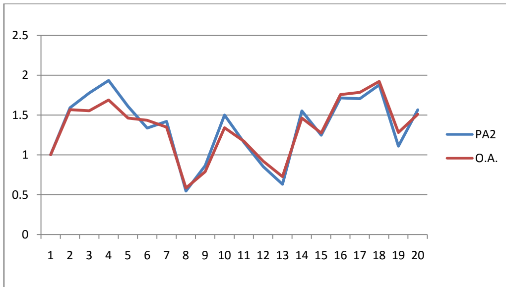
Fig 3. Graphical presentation of Best Model (PA2) of set B.
