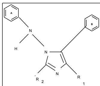
Figure 1. Parent skeleton of Anti-HIV 5-phenyl-1-H-imidazole
