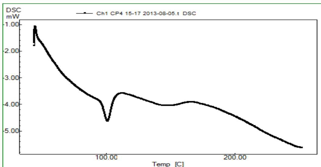
Figure 1: DSC spectra of Chlorpheniramine Maleate
