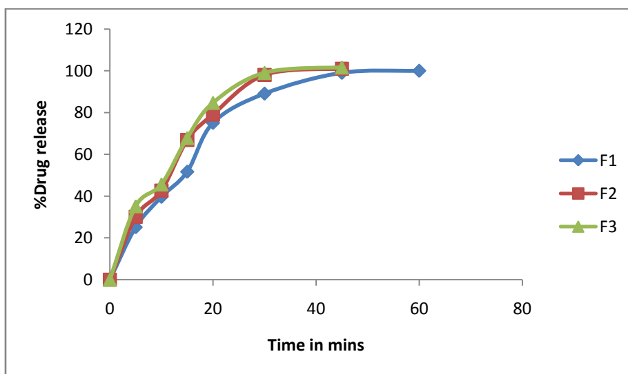
Figure 5:- Percentage cumulative drug release profile of Chlorpheniramine Maleate.
