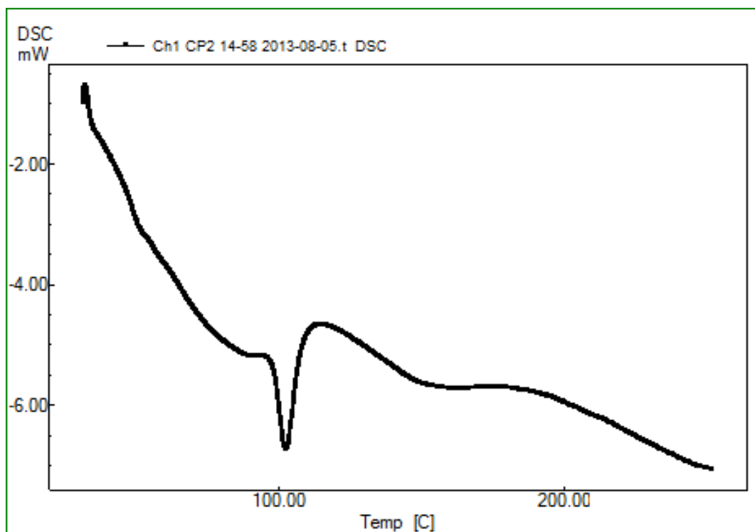
Figure 2: DSC spectra of Medicated chocolate (Chlorpheniramine Maleate + Chocolate base).
